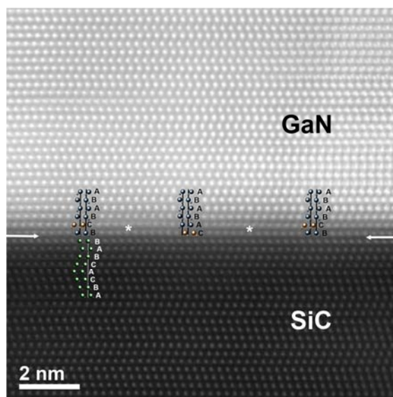
Figure 7: HAADF-HRSTEM image of the GaN-SiC interface. A model of stacking sequence in SiC is also inserted. The white arrows mark the interface. The asterisks mark the areas in GaN where the stacking sequence from BCB to CAB and back is changing.
