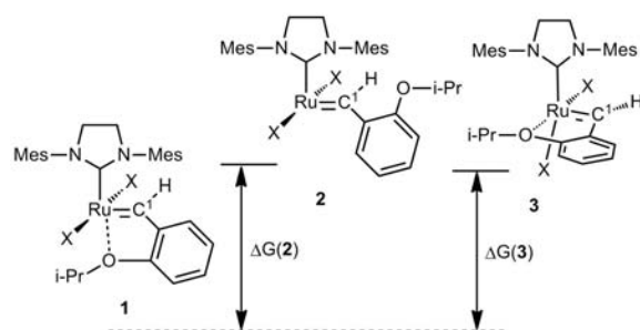
Figure 2: Three stable structures 1 - 3 of the initiator. The most stable structure (1) is stabilized through Ru-O interaction.
