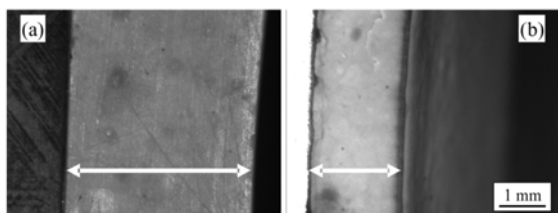
Figure 2: TMS images of an outer ceramics wall of the SPT-100D EM1 at the beginning (a) and at the end (b) of the test campaign. The top plane of the ceramics walls is indicated by double arrows.
