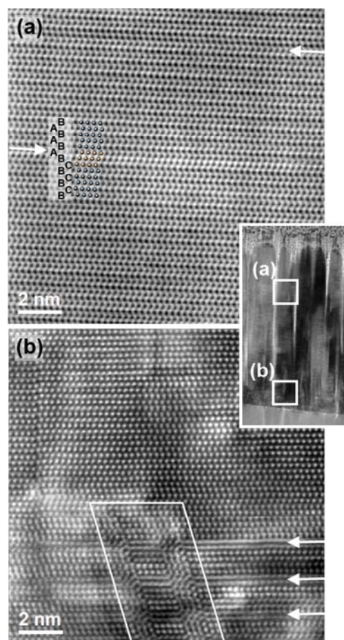
Figure 6: (a) High-resolution BF-STEM image (Wiener filtered) of an area close to the top of the porous GaN film with two stacking faults (white arrows). (b) High-resolution HAADF-STEM image of the film close to the SiC substrate with cubic GaN inclusions and stacking faults (white arrows).
