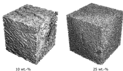
Figure 4: \mu CT studies of PEG cryogels independence on the monomer concentration.
