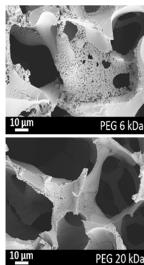
Figure 6: Influence of PEGs as pore forming agents on the porosity of PEG cryogels [3].
