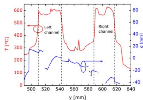
Figure 4: Pyrometer (solid line) and TLH scan (dashed line) across the diameter of the SPT-100D EM1. The scans are recorded immediately after switching-off the thruster which is operated at U = 750 \text{ V} and I = 2.6 \text{ A} . The thruster is tilted by 25^\circ . The vertical dotted lines mark the left and right plasma channel.
