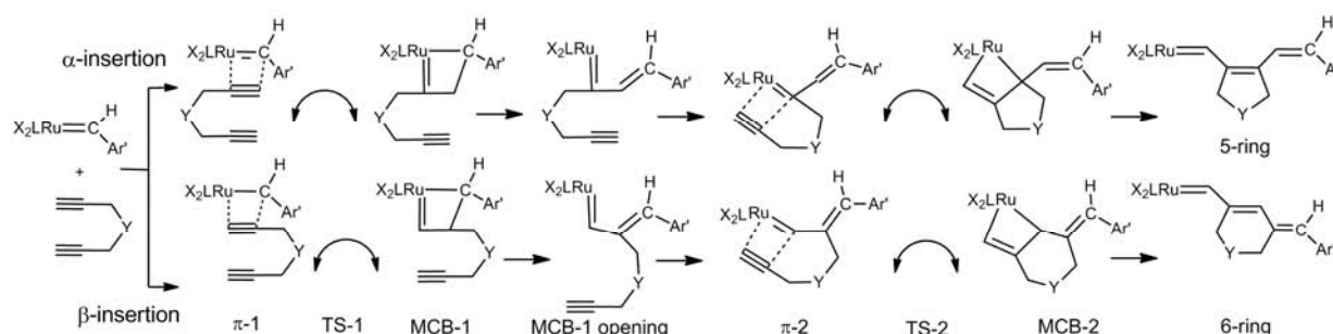
Figure 1: The two possible reaction pathways ( \alpha - and \beta -insertion) leading to the formation of five- and six-membered repeat units.
