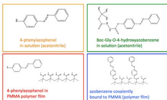
Figure 1: Systematic study of light induced cis-trans isomerization dynamics of azobenzene in four different systems.
