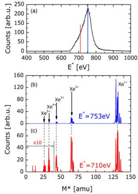
Figure 6: ESMS energy scan (a) and mass scans (b,c) of the SPT-100D EM1 operated at U = 750 V and I = 2.6 A. The mass scans are measured at two energies as indicated in panel (a) ( E^* = 753 eV, E^* = 710 eV).
