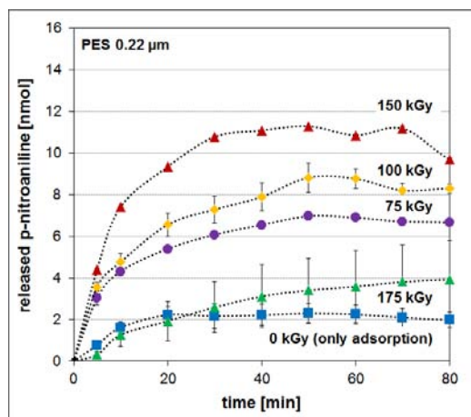
Figure 2: Trypsin activity after immobilization on a polyethersulfone (PES) membrane with different electron beam doses.
