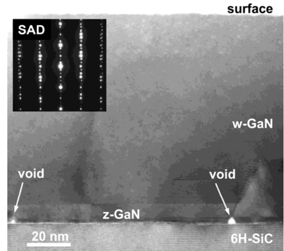
Figure 3: TEM micrograph of an almost 100 nm thick GaN film prepared by ion-beam nitridation of Ga droplets. The SAD pattern (inset) originates from the film-substrate interface region.
