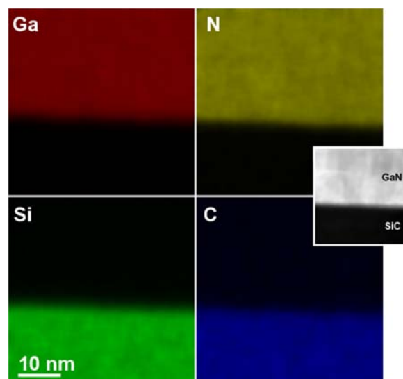
Figure 3: EDX elemental maps of Ga, N, Si and C element distributions at the GaN-SiC interface. The inset shows the STEM image of the acquired area.
