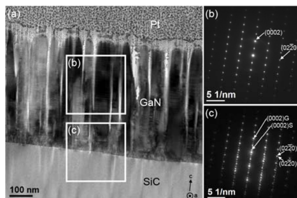
Figure 4: (a) Bright-field TEM micrograph of a porous GaN film grown on 6H-SiC(0001) at a substrate temperature of 750 °C taken at 80 kV acceleration voltage. (b) and (c) electron diffraction patterns of the film and the interface region, respectively.
