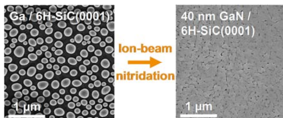
Figure 2: SEM micrographs of Ga droplets formed on a 6H-SiC(0001) substrate surface (left) and a GaN thin film obtained after hyperthermal ion-beam nitridation of such droplets (right).
