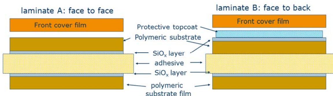
Figure 1: Schema of the face-to-face (left) and the face-to-back (right) lamination of two mono-layer barrier films.
