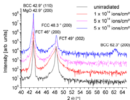
Figure 1: XRD measurements showing the FCC to FCT phase transformation for 10^{14} ions/cm 2 and the transformation to BCC for 5 \times 10^{15} ions/cm 2 .
