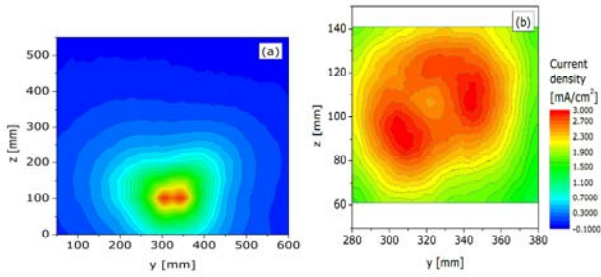
Figure 5: Current density maps of the SPT-100D EM1 operated at U = 750 V and I = 2.6 A measured with the Faraday probe at a distance of d = 600 mm. Panel (a) shows a map plotted from horizontal line scans measured at \Delta z = 50 mm, panel (b) is a centre map with \Delta z = 2 mm and a reduced y -range.
