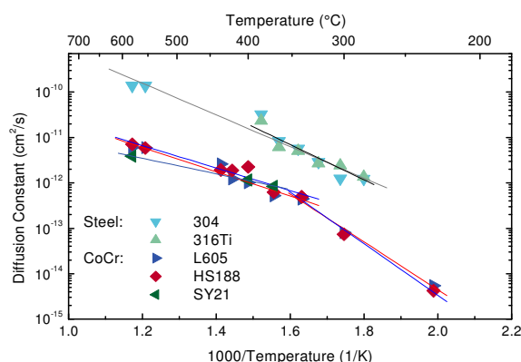
Figure 1: Arrhenius plot of resulting diffusion constants as a function of temperature for three CoCr alloys as well as two stainless steel alloys.
