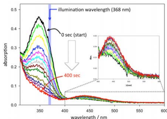
Figure 2: Change of absorption spectrum of 4-phenylazophenol in PMMA polymer film during illumination with 368 nm light. The change in absorption directly reflects the light induced switching from trans to cis isomer.
