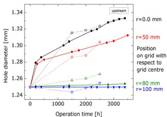
Figure 8: Comparison between measured (open symbols) and simulated (closed symbols) accelerator grid hole diameters of a RIT-22 for different radial positions of the hole on the grid.
