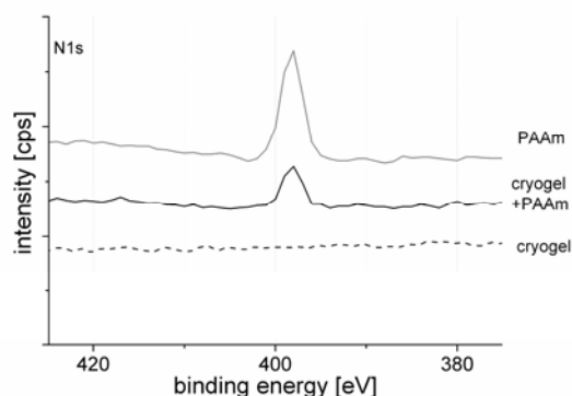
Figure 7: Proof of the successful incorporation of amine groups by XPS [2].
