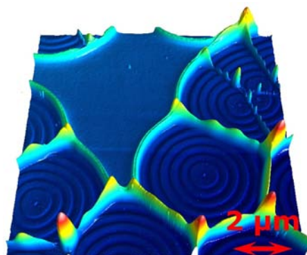
Figure 2: 3D AFM image of an irradiated 10 nm Cr/SiO 2 system (laser fluence \Phi = (250 \pm 50) \text{ mJ/cm}^2 , number of laser pulses N = 6 ).
