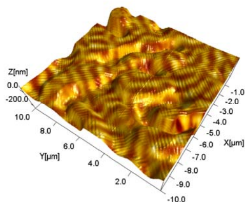
Figure 2: Stacked AFM and MFM image of a martensitic FCT \text{Fe}_7\text{Pd}_3 sample. Different magnetic domains (yellow and red), run predominantly perpendicular to the martensitic twinning boundaries.
