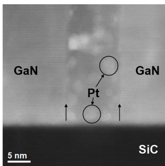
Figure 5: Cross-sectional HAADF-STEM image of a pore in a GaN thin film. The arrows indicate the sidewalls of the pore which occurs directly at the 6H-SiC substrate surface.
