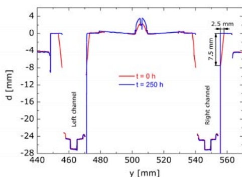
Figure 3: TLH line scans across the centre of the SPT 100D EM1 at the beginning (a) and at the end (b) of the test campaign.
