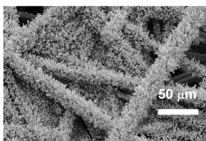
Figure 1: \text{CsH}_2\text{PO}_4 nanoparticles deposited via a nano-spraydryer, directly on a solid acid fuel cell current collector.
