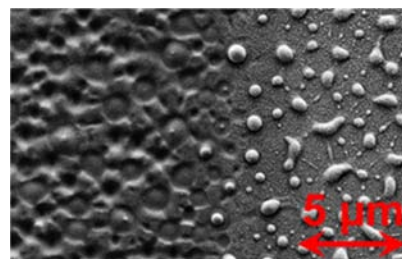
Figure 3: SEM image of an irradiated 20 nm Cr/SiO 2 sample; (right) only the pre-structured metal layer (Step 1: \Phi = (200 \pm 50) \text{ mJ/cm}^2 , N = 5 ) and (left) the structured fused silica surface (Step 2: \Phi = (300 \pm 50) \text{ mJ/cm}^2 , N = 9 ).
