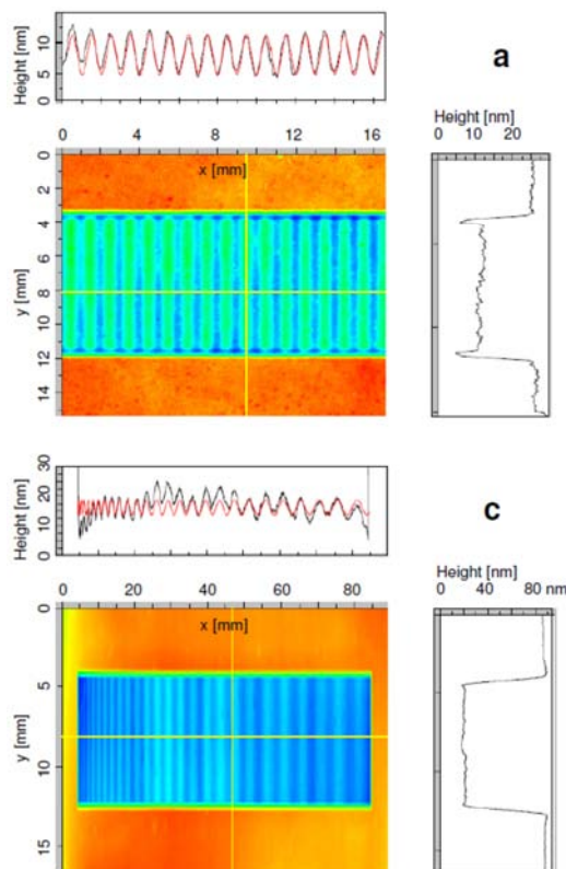
Figure 1: (a) Plasma jet generated sinusoidal surface profile with period of 1 mm and PV of 5 nm, (c) chirped profile.
