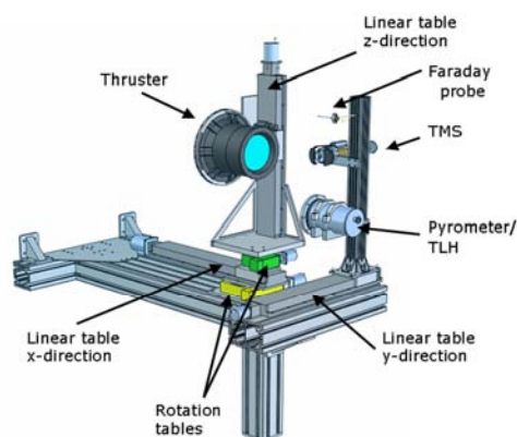
Figure 1: Drawing of the diagnostic system with 5-axis positioning system, diagnostic heads and a thruster. Not shown is the ESMS, which is mounted to one of the chamber walls.
