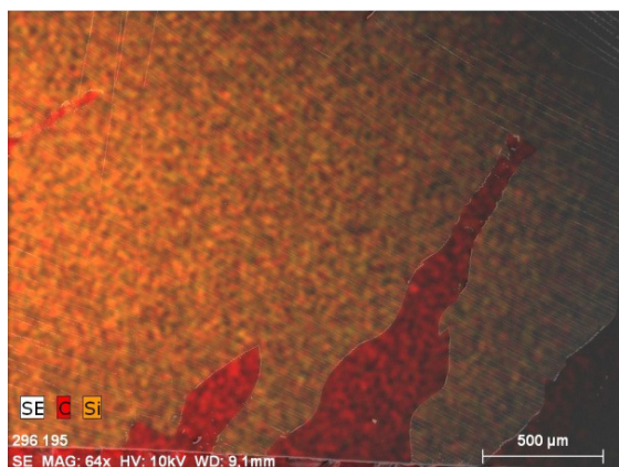
Figure 6: SEM-EDX image of the delaminated interface protecting topcoat – silica layer showing that the silica layer remained almost completely on the top of the PET substrate.
