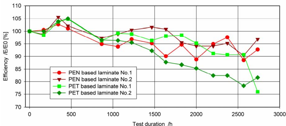
Figure 5: Results of the combined climate test consisting of alternating damp-heat and thermo-cycle exposure including wetting and freezing.
