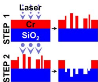
Figure 1: Schematic illustration of the IPSM-LIFE process (STEP 1: low fluence, STEP 2: high fluence treatment).
