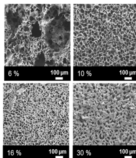
Figure 3: Effect of the concentration on the cryogel morphology [2].
