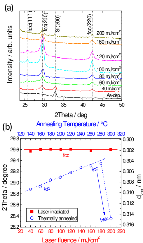
Figure 1: Laser crystallization of GST-films showing (a) T2T-measurement for samples crystallized with different fluence and (b) lattice parameter dependence on laser fluence and annealing temperature.
