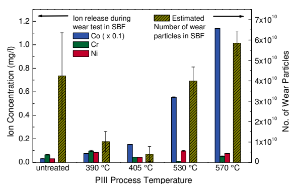
Figure 4: Comparison of metal ion release during wear tests in SBF with number of wear particles. Please note that the cobalt concentrations were multiplied by a factor of 0.1 for clarity.
