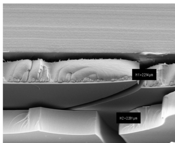
Figure 2: SEM image of laminated barrier films.
