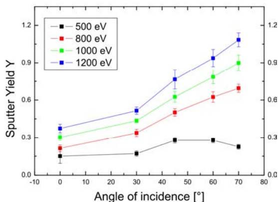
Figure 7: Graphite sputter yield in dependence on the angle of incidence and energy of the Xe-ions.
