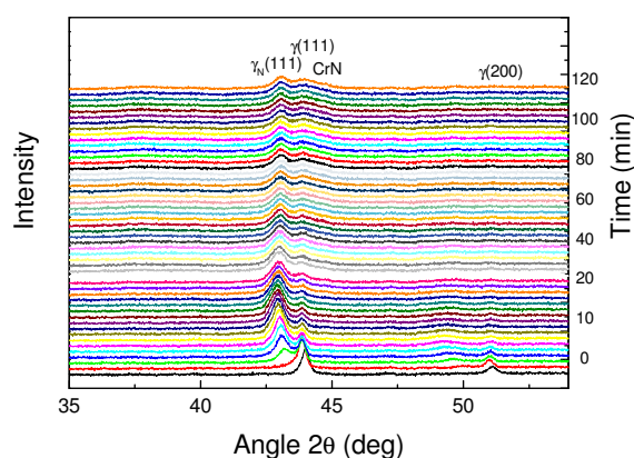
Figure 3: Time evolution of XRD spectra during low energy nitriding at 550 °C.
