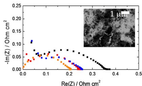
Figure 2: Impedance spectra for four separate symmetric cells CNT-Electrode/ \text{CsH}_2\text{PO}_4 /CNT-Electrode, measured at 240^\circ\text{C} and \text{O}_2 atmosphere. Inset showing SEM image of as grown, catalytically active CNTs. [3]
