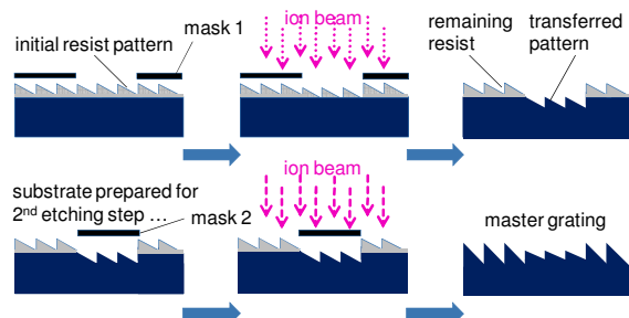
Figure 1: Modified transfer process of the resist pattern by integration of complementary structured masks.
