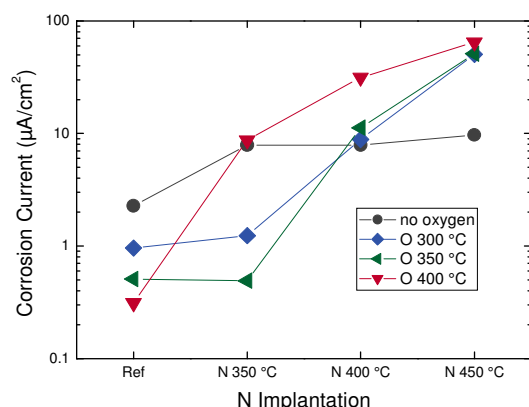
Figure 5: Corrosion rates calculated from the polarisation curves as function of nitrogen and oxygen implantation temperature. The samples labelled as "ref" are only implanted with oxygen (with indicated temperature), together with a sample from untreated base material (black circle).
