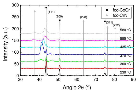
Figure 2: XRD spectra for CoCr alloy HS188 after nitrogen PIII for temperatures between 230 °C and 580 °C.
