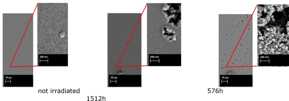
Figure 1: Scanning electron microscopy images displaying the development of the destruction of a commercial coating CET6 (Cetelon, Germany) by UVA irradiation with added 1% P25.
