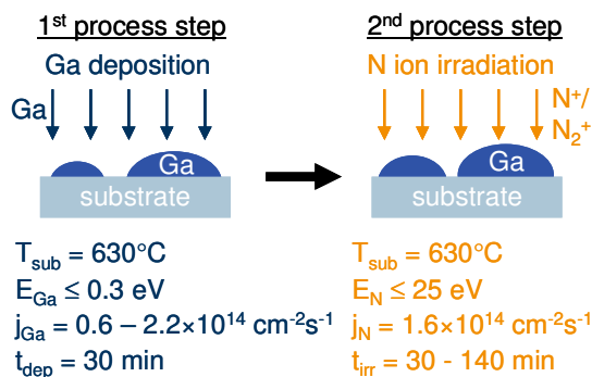
Figure 1: Schematic of the investigated two-step process and typical preparation parameters.
