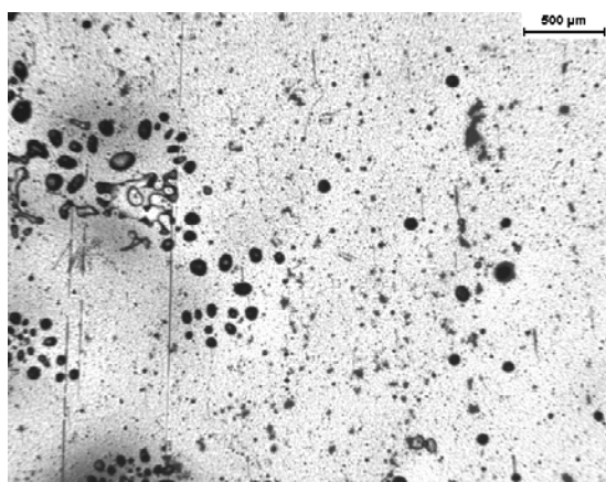
Figure 3: Image of a barrier film after Ca test - visualization of defects.
