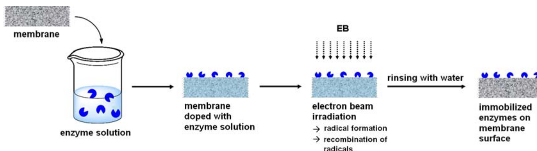
Figure 1: Procedure for the coupling of trypsin on polymer membranes using electron beam irradiation.
