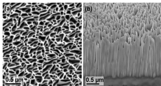
Figure 1: (a) SEM image of porous GaN thin film. (b) FIB cross-section of the sample shown in (a).
