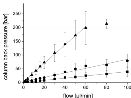
Figure 5: Column back-pressure of cryogel capillaries (ID=200 \mu m) in dependence on the (macro)monomer concentration [2]. Triangle: 25wt.%, filled circles: 15wt.%, filled squares: 10wt.%.
